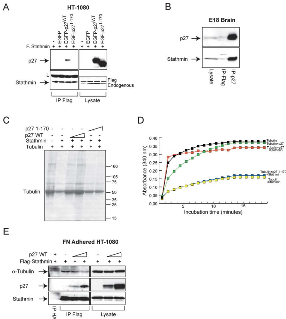
Figure 3. p27 binds and inhibits the MT-destabilizing protein stathmin
